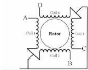
Unipolar Stepper Motor
