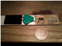
832. Ultra low cost solar-rechargeable persistence of vision display using PIC10F206 Ultra low cost solar-rechargeable persistence of vision display This device produces a big eye catching display to write text and small images through the air. It uses under £2 (approx $3.20 US at the time of writing) of parts, and is a nice little..... Listed under: LED Projects, Projects
